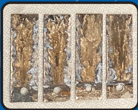
Controls (Untreated Al Alloys - 7075-T6)
